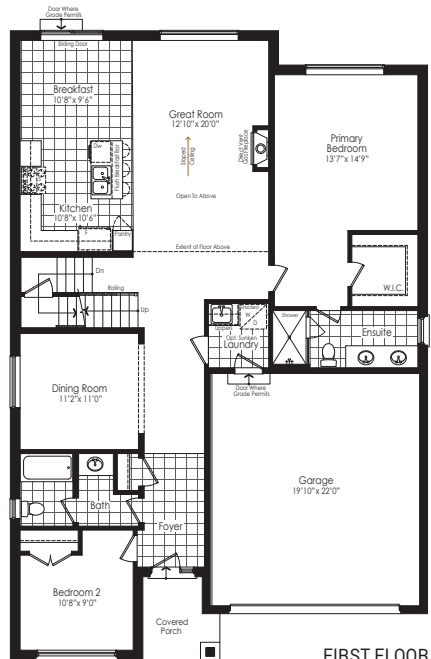
FIRST FLOOR ELEVATION A & B OPT. 4 BEDROOM PLAN
