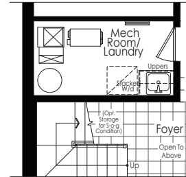
FIRST FLOOR (SLAB ON GRADE) ELEVATION B
