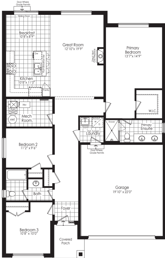
FIRST FLOOR (SLAB ON GRADE) ELEVATION A & B
