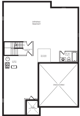
BASEMENT ELEVATION A & B
