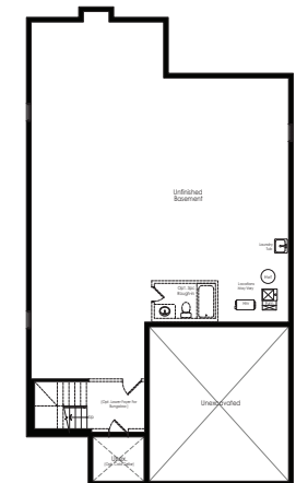
BASEMENT ELEVATION B
